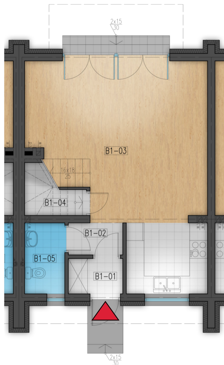
parter
